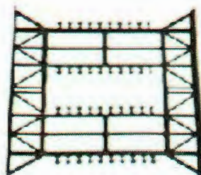
Figure 1 – Advantage ICF System Web Connector
